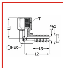
內牙插心彎頭 Female Hose-Barb Elbow
