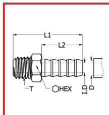
惠氏牙插心接頭 Whitworth male Hose-Barb Connector
