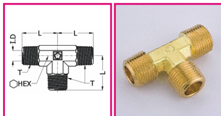
外牙三通 Male Tee
