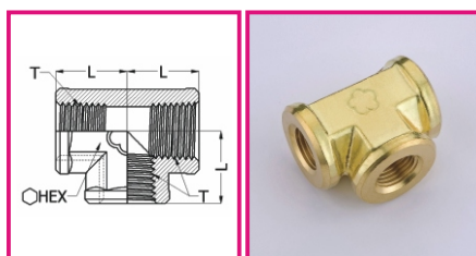
內牙三通 Union Tee
