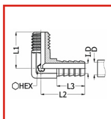
惠氏牙插心彎頭 Whitworth male Hose-Barb Elbow
