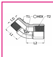
45°內外彎頭 45° Street Elbow
